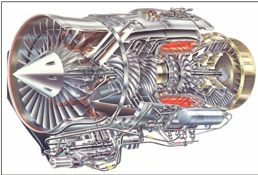
Cross sectional view of F-109 Jet Engine
